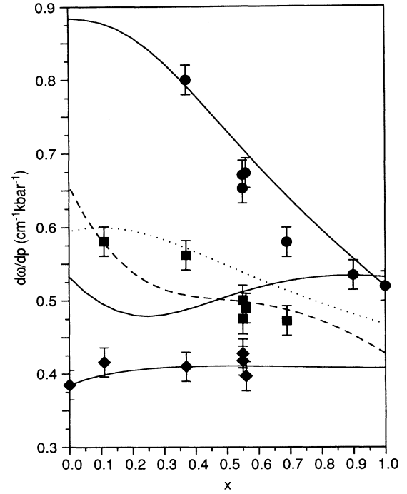
FIG. 3. d\omega_i/dp as a function of the Si fraction x for the Si-Si (circles), Ge-Si (squares), and Ge-Ge (diamonds) modes. The solid lines are calculated by using the CI model with dZ/dp = 0 for the Ge-Si mode. The dashed curve for the Ge-Si mode is a fit to the CI model with dZ/dp = -180 \text{ cm}^{-2}/\text{kbar} , and the dotted curve for the Ge-Si mode is fit by using the simple model of Eq. (11).
